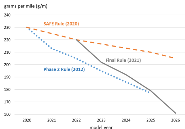
Figure 2. EPA Fleet-Wide CO 2 Compliance Targets, MY2020-2026
