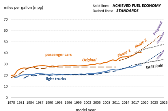
Figure 1. CAFE Standards and Achieved Fuel Economy
